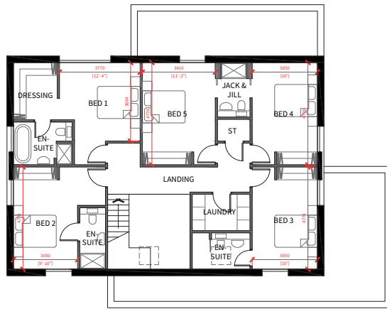
1F First Floor Plan 1:75 @ a1
