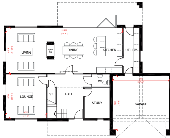
GF Ground Floor Plan 1:75 @ a1
