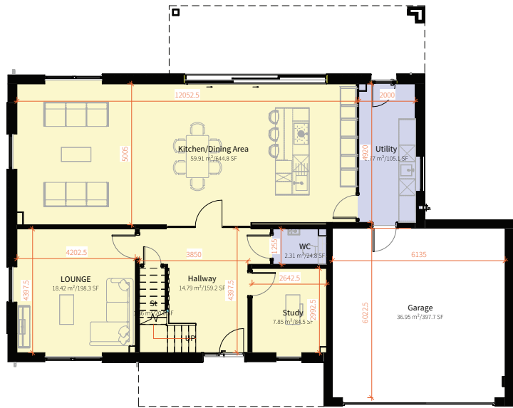
1 GA_Plan_00-Ground 1:100
