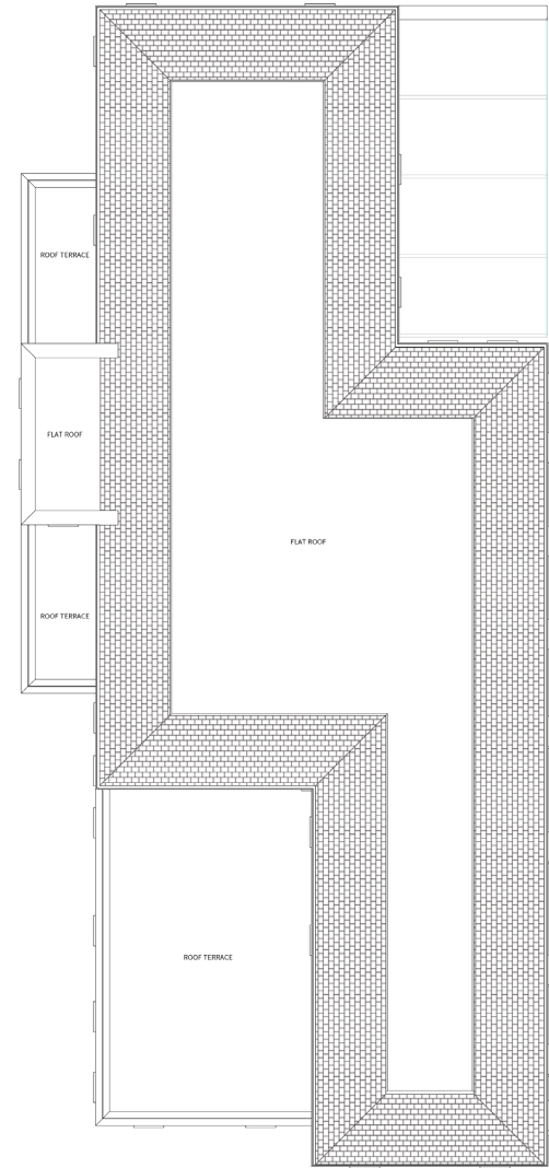
3 GA_Plan_Roof 1:100
