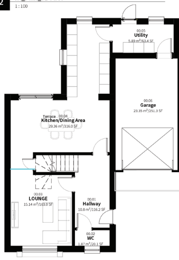
1 GA_Plan_00-Ground 1:100
