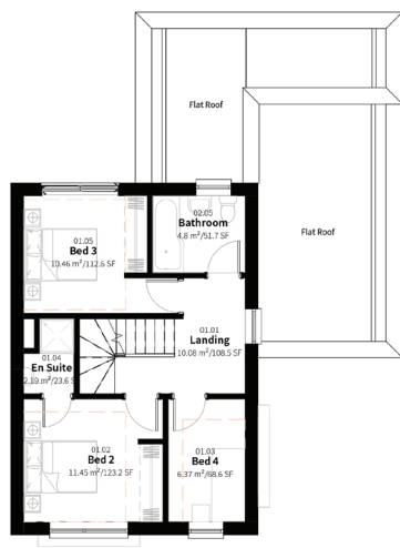
2 GA_Plan_01-First 1:100
