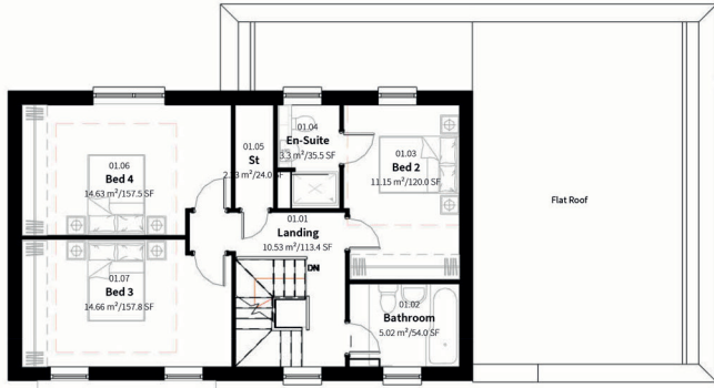
2 GA_Plan_01-First 1:100
