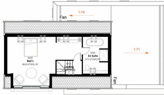
3 GA_Plan_02-Second 1:100
