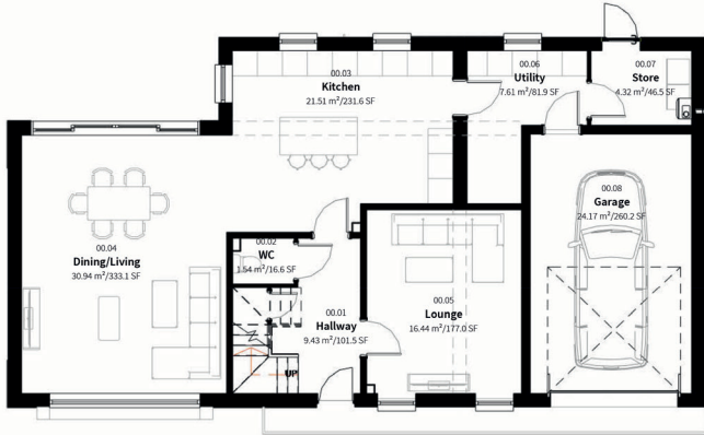
1 GA_Plan_00-Ground 1:100
