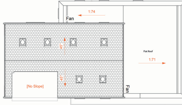
4 GA_Plan_Roof 1:100
