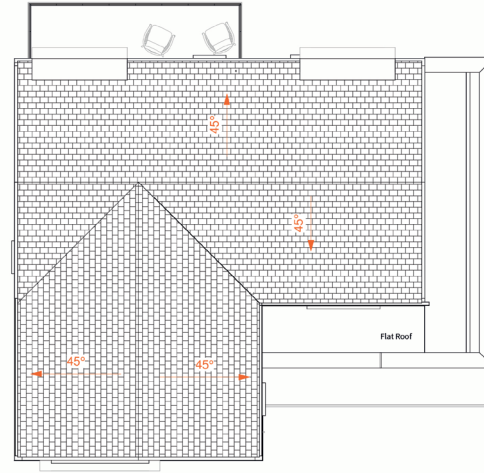
4 GA_Plan_Roof 1:100
