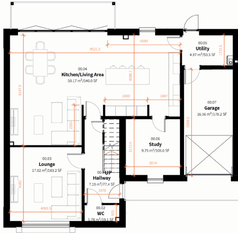
1 GA_Plan_00-Ground 1:100
