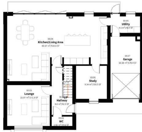
1 GA_Plan_00-Ground 1:100
