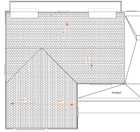
4 GA_Plan_Roof 1:100
