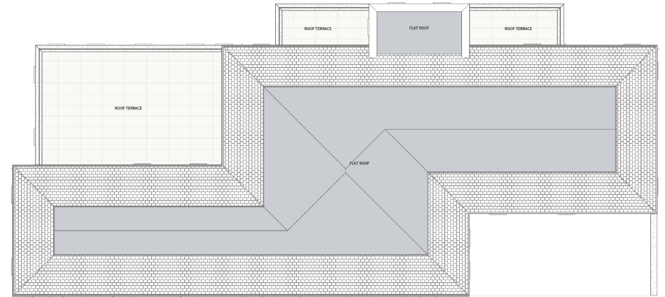
3 GA Plan_Roof 1:100
