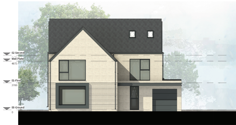
1 GA_Elevations_Front 1:100
