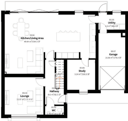
1 GA_Plan_00-Ground 1:100
