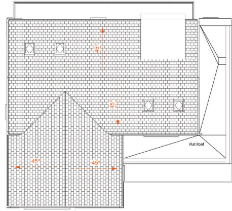
4 GA_Plan_Roof 1:100
