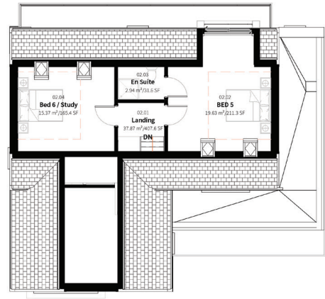
3 GA_Plan_02-Second 1:100
