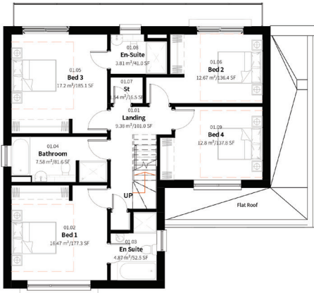
2 GA_Plan_01-First 1:100
